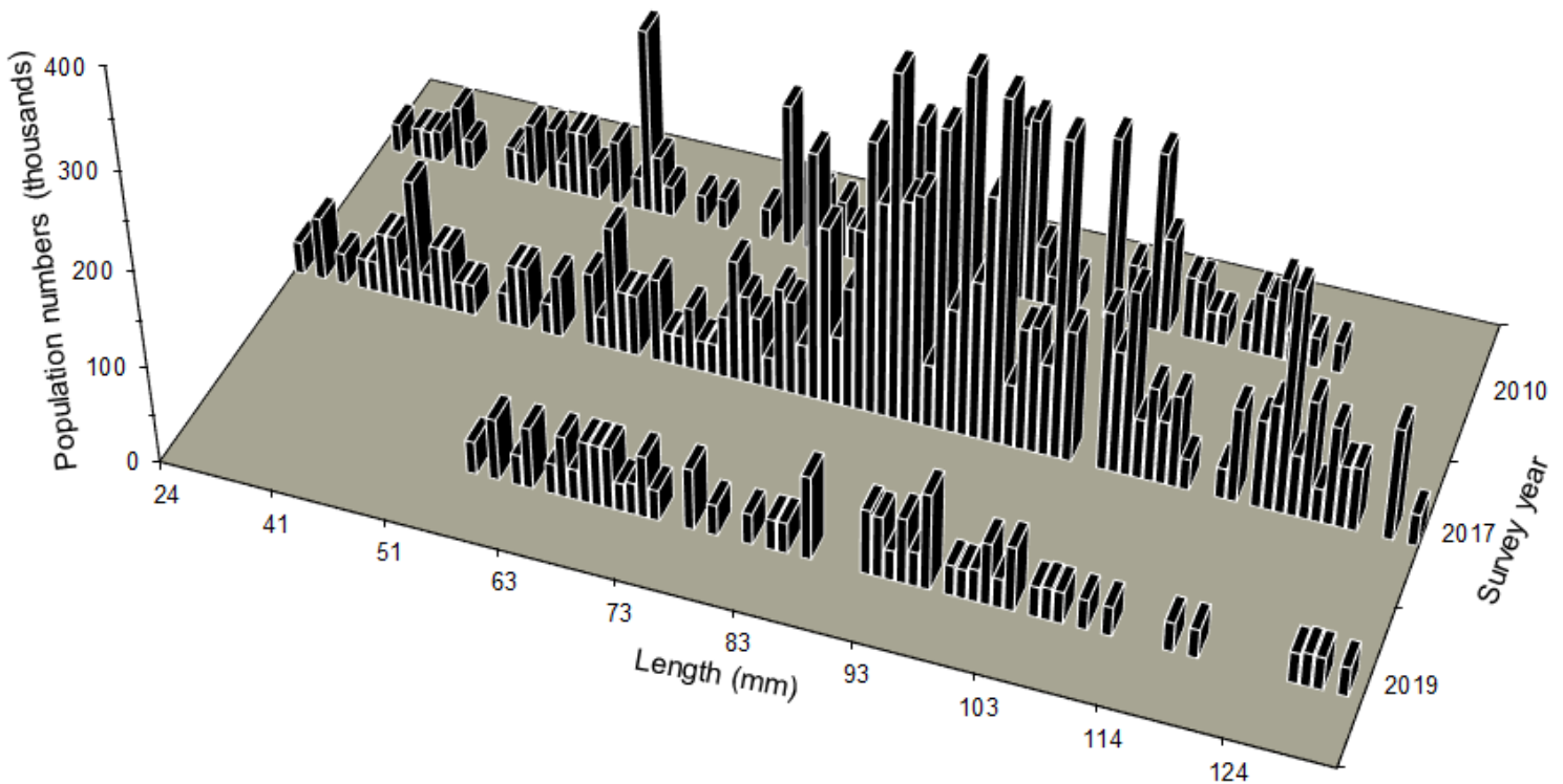
Figure 31. Total abundance-at-size of blue king crab in the NBS during 2010, 2017 and 2019.
