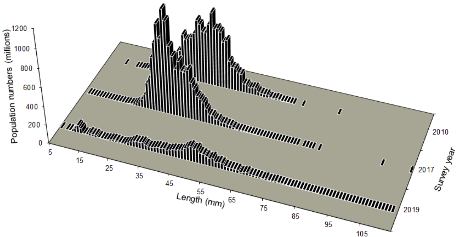
Figure 9. Total abundance-at-size of snow crab in the NBS during 2010, 2017 and 2019.
